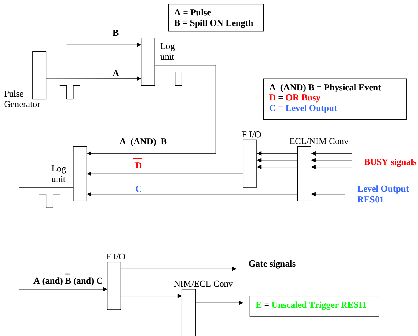
Fig. 3. Trigger : electronic scheme
