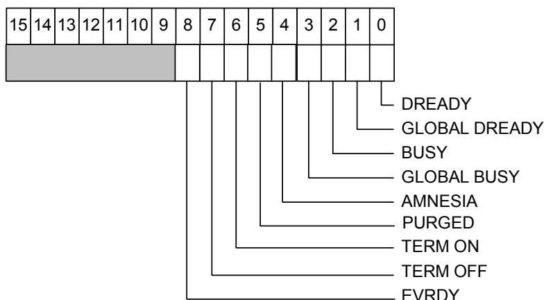
Fig. 4.15: Status Register 1
