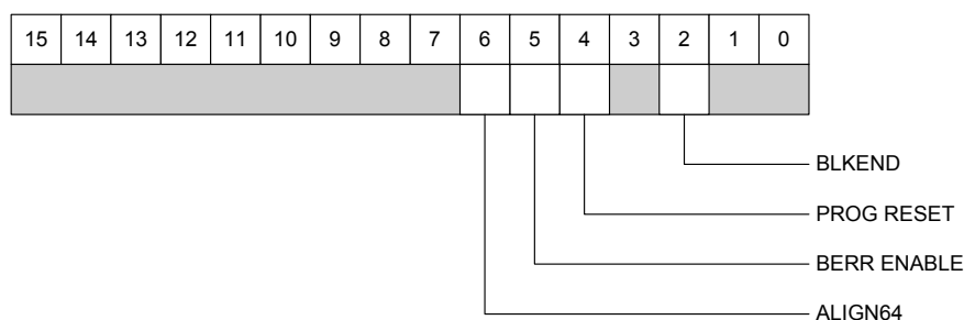
Fig. 4.16: Control Register 1
