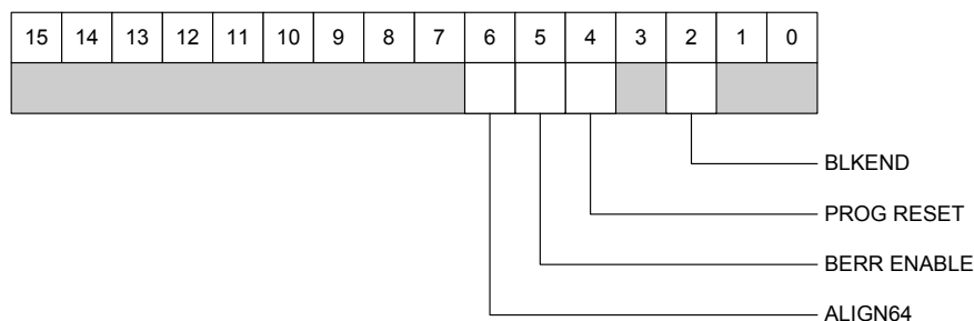
Fig. 4.17: Control Register 1
