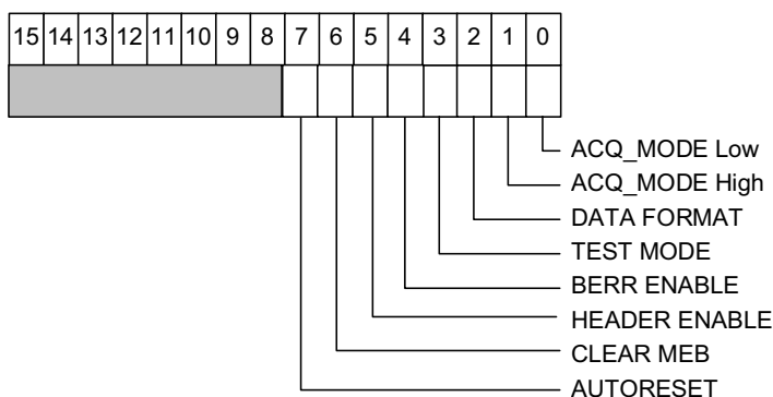
Fig. 3.8: Control Register
