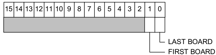
Fig. 3.18: MCST Control Register
