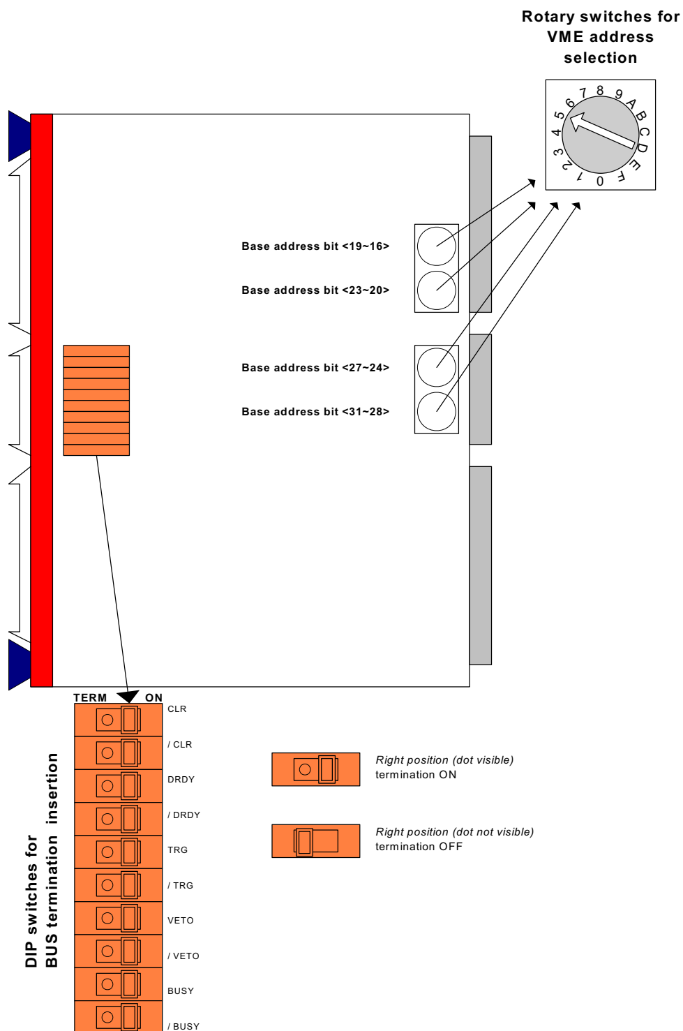
Fig. 2.4: Components Location (components side)
