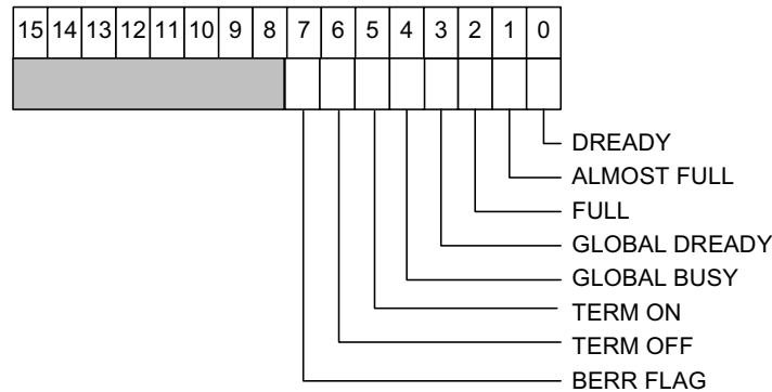
Fig. 3.10: Status Register
