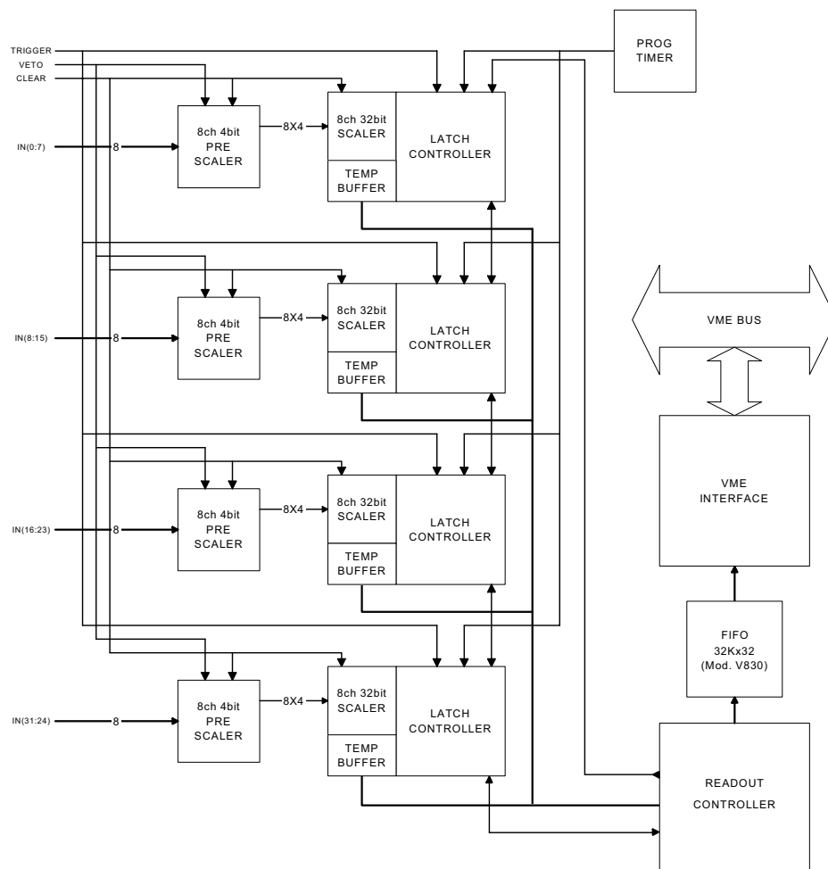
Fig. 1.2: Model V820/V830 Block Diagram
