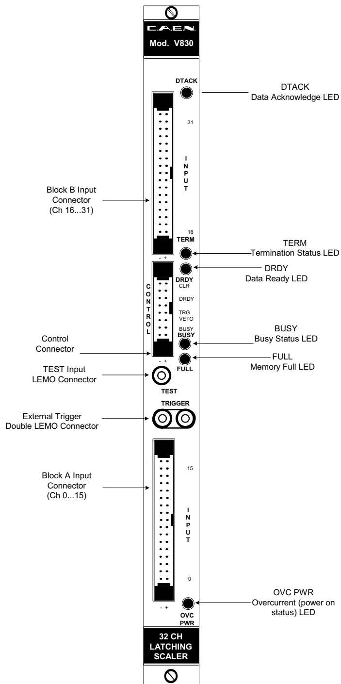
Fig. 2.1: Model V820/V830 front panel
