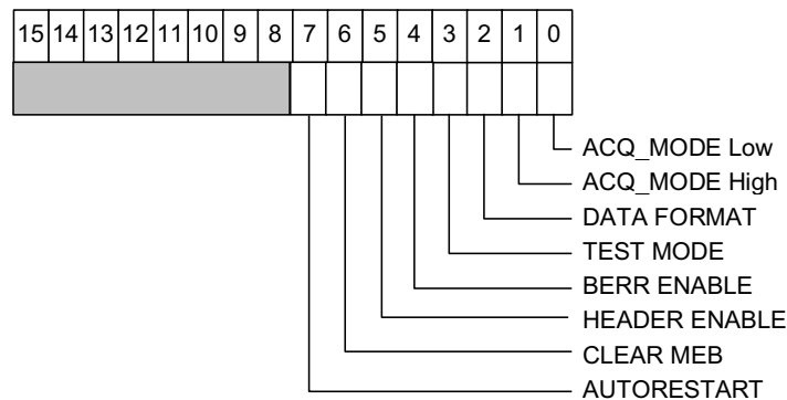
Fig. 3.9: Control Bit Set Register
